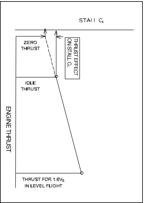
FIGURE 29-5. THRUST EFFECT ON STALL C_L
